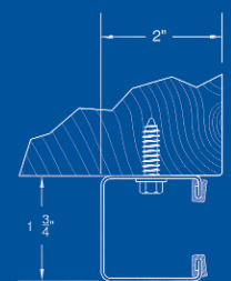
WOOD JAMBS
