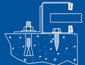
Masonry Mount
